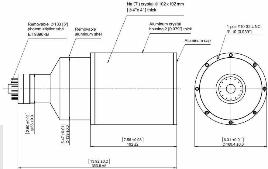
Model 24S24/5
