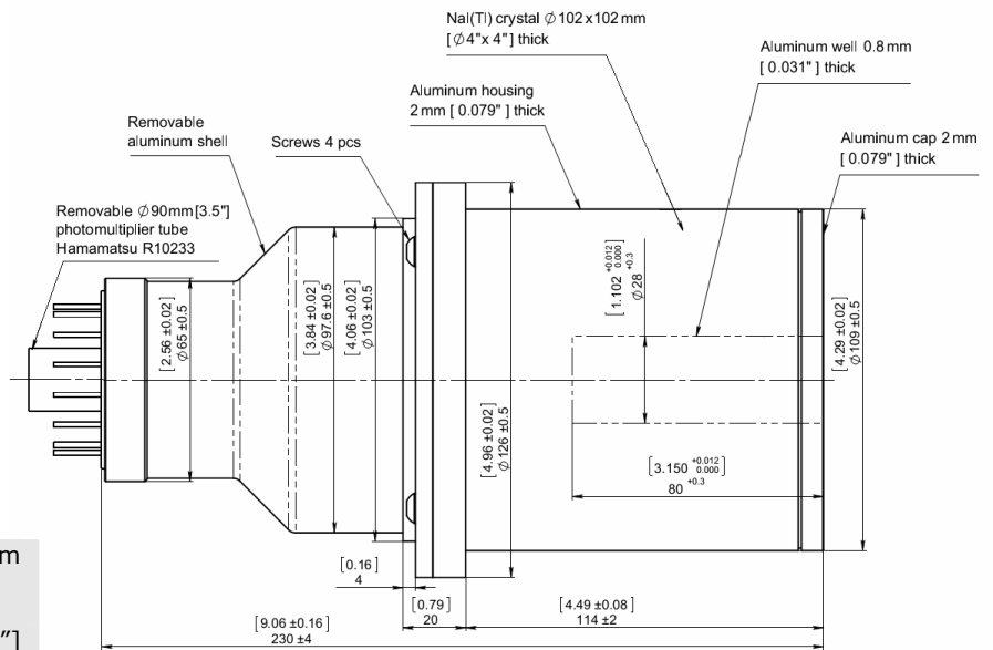
Model 16SW16/3.5.C2
